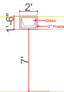
V24 2'-0"X1'-6" Frame size=3"x2"
