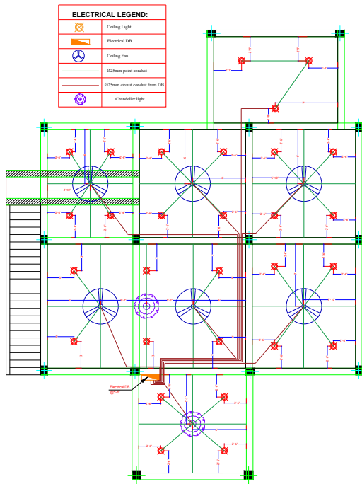
FLOOR PLAN - SLAB ELECTRICAL
