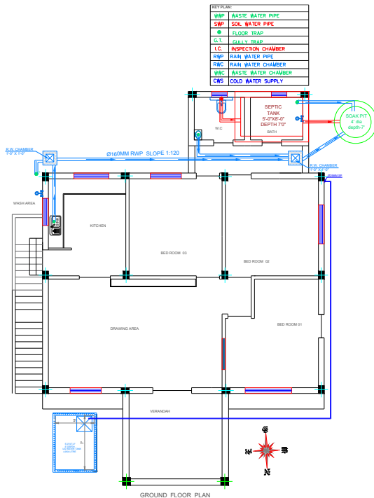
FLOOR PLAN - PLUMBING & DRAINAGE
