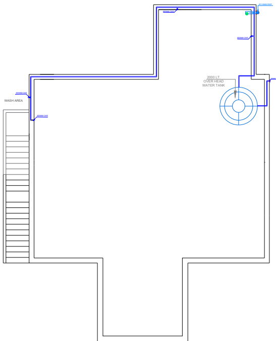
TERRACE FLOOR PLAN - PLUMBING & DRAINAGE
