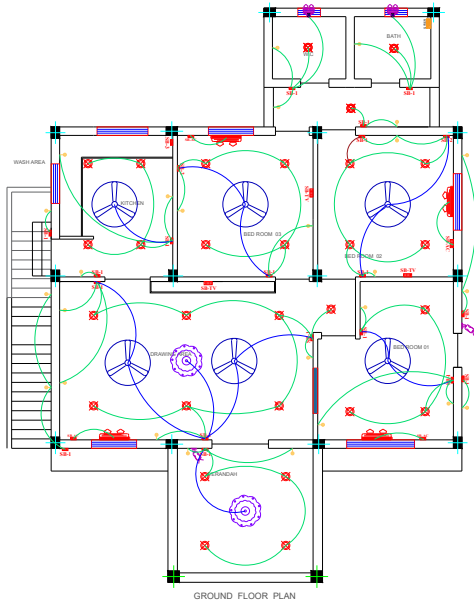
FLOOR PLAN - DETAILS ELECTRICAL
