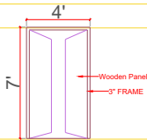
D48 4'-0"X7'-0" Frame size=5"x3"
